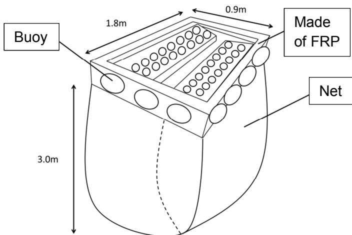
Structure of the trap used for capturing seals
